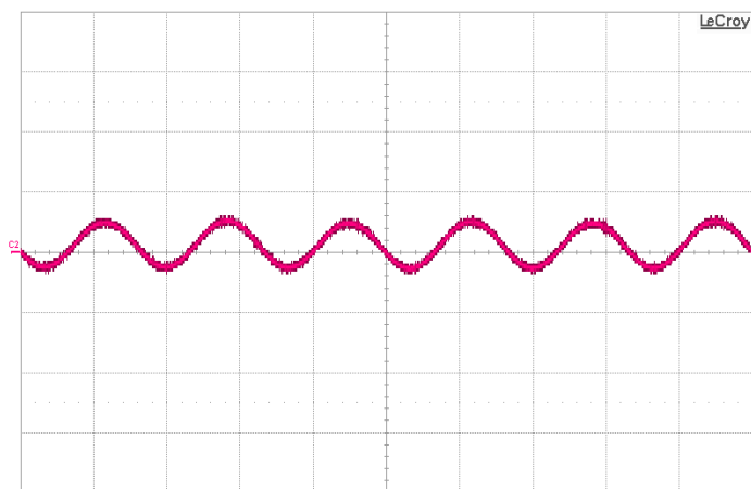
Figure 7: Output voltage with 500µF Hold-up capacitor at full rated power (115VAC, 60Hz) Red: Vout (10V/div), Timebase: (5ms/div)
